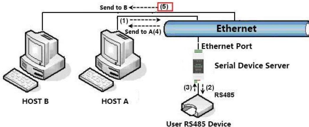
Figure 36 Multi-host function demonstration
