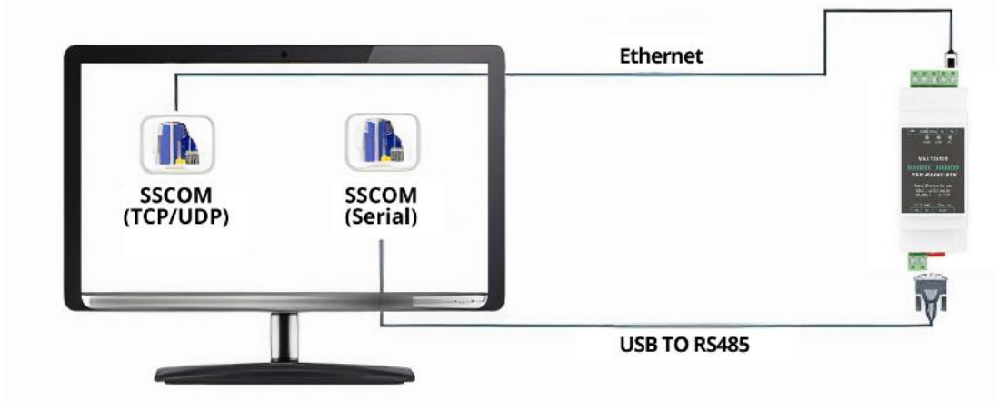
Figure 9 TCP communication diagram
