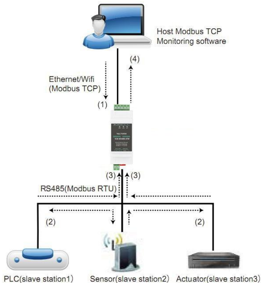
Figure 34 Storage Modbus Gateway
