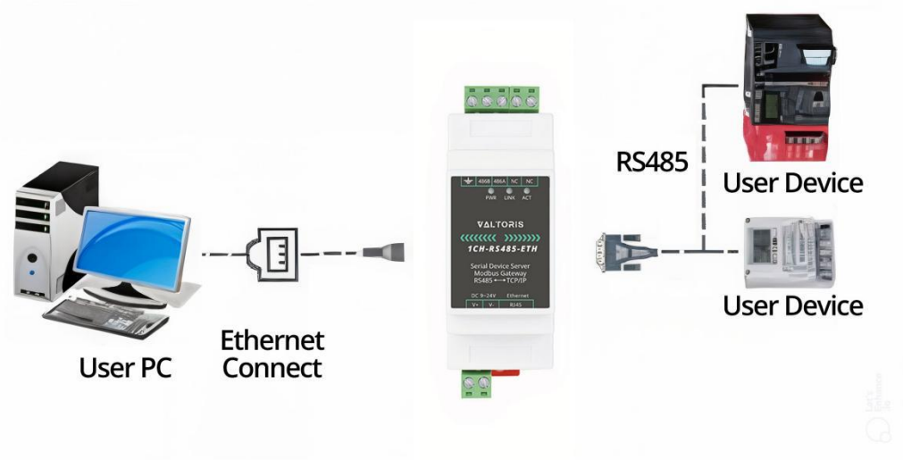
Figure 2 Connection Diagram
