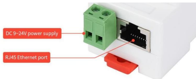
Figure 4 power supply and network port
